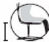
seat height 460 - 580
